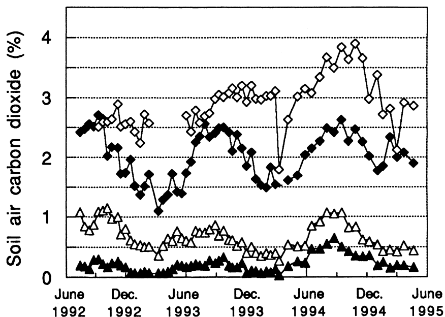
Figure 5. Seasonality of soil carbon dioxide illustrated by mean concentrations from four soil depths in four or eight permanent plots in the Calhoun soil profile. ▲ is carbon dioxide concentrations of soil at 0.15 m, Δ is concentrations at 0.6 m, ◆ is concentrations at 1.75 m, and ◇ is concentrations at 4.0 m.
