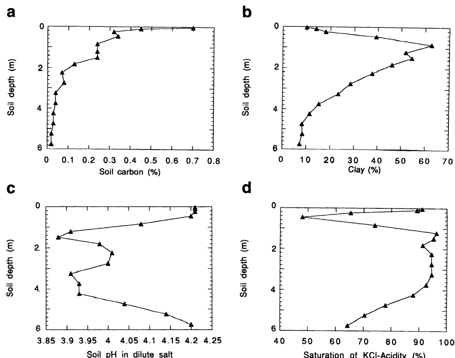
Figure 2. Soil properties often vary in regular patterns with depth. The illustrated example is the Ultisol soil of the South Carolina Piedmont at the Calhoun Experimental Forest. The Ultisol soil is old and highly weathered. (a) Soil organic carbon has a steep gradient with depth, decreasing from 0.7% in the upper 7.5 centimeters of the A horizon down to approximately 0.03% in the C horizon at more than 4-meter depth. With increasing depth, the soil carbon is increasingly old; the soil carbon at more than 2 m has an equivalent ^{14}\text{C} -age of 4500 to 8000 years since photosynthetic fixation. (b) Percentage of clay has a maximum (63%) in the B horizon and is much lower above and below this depth. Clay moves from the A and E horizons to accumulate in the B horizon. In this Ultisol soil, the clay is predominantly a crystalline mineral known as kaolinite and is highly acidic with iron-oxide coatings. These iron-oxide-rich clays are common to many of the world's most weathered soils and are resistant to further weathering and decomposition. (c) The Calhoun soil is low in pH (less than 4.2) throughout the entire 6-meter profile. In contrast, the granite-gneiss bedrock from which these soils are derived has a pH of 7.9. (d) Soils have large amounts of exchangeable acidity. Soil clays and organic matter have a primarily negative charge, known as cation exchange capacity (CEC), which attracts and adsorbs nutrient and acidic cations (positive ions). In low-fertility Ultisols, few of these adsorbed cations are nutrients, most are acids. In the extremely acidic Appling soil, much of the profile has more than 90% of its negative charge balanced by acids.
